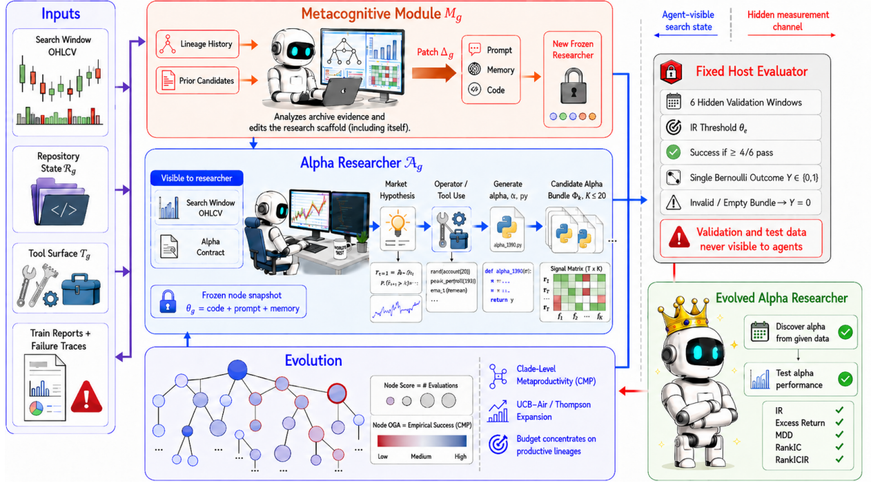
Figure 1 Overview of STAR. STAR evolves an alpha researcher rather than only individual alpha formulas. At each archive node, a frozen researcher snapshot (consists of (code_a, prompt_a, memory_a) ), receives search-window OHLCV data and alpha contract, then emits candidate alpha programs. A fixed host evaluator scores bounded candidate bundles on hidden validation windows and converts each admitted call into a single binary success observation. A metacognitive module reads only train-side lineage information and reports, then patches the state of the researcher or itself to create a child node. Clade-level metaproductivity allocates evaluation and modification budget toward lineages whose descendants repeatedly produce better alphas. Final evolved alpha research policies at budget exhaustion obtain stronger capability in generating high quality alphas.
